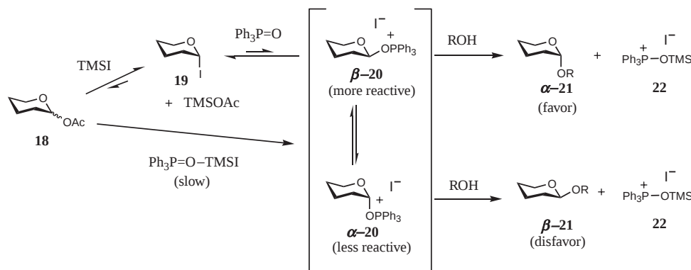
Scheme 2. Reaction mechanism of glycosylation with glycosyl acetate by the promotion of TMSI and \text{Ph}_3\text{P}=\text{O} via glycosyl phosphonium iodide.
