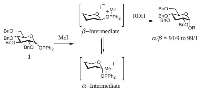
Scheme 1. Glycosylation of glycosyl acceptor with donor 1 and iodomethane.
